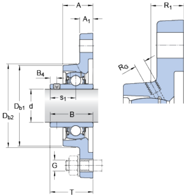
FYT 15/16 TF Bearing 2D drawings and 3D CAD models
